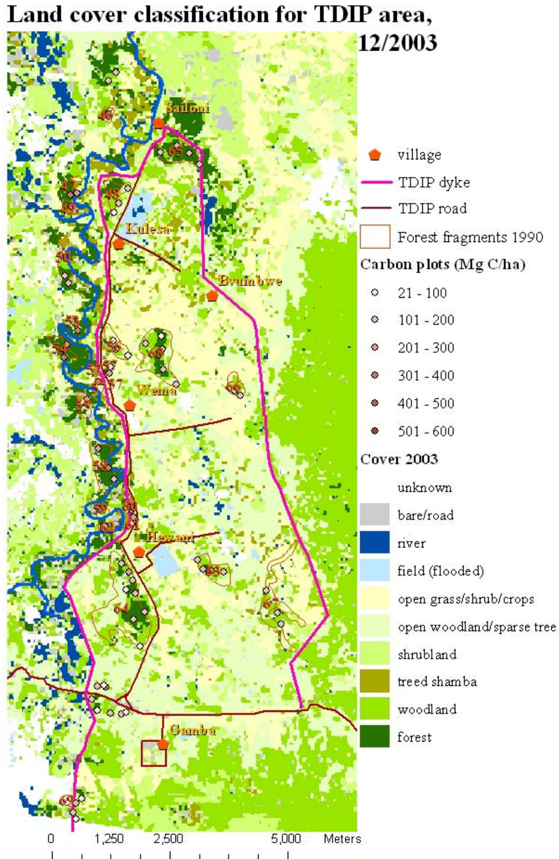
Figure 2 Map of supervised spectral classification of Landsat ETM, 166/61, 12/2003. Inventory plot locations based on GPS readings. Dyke, road, and forest fragments from digitization of TARDA TDIP maps.
