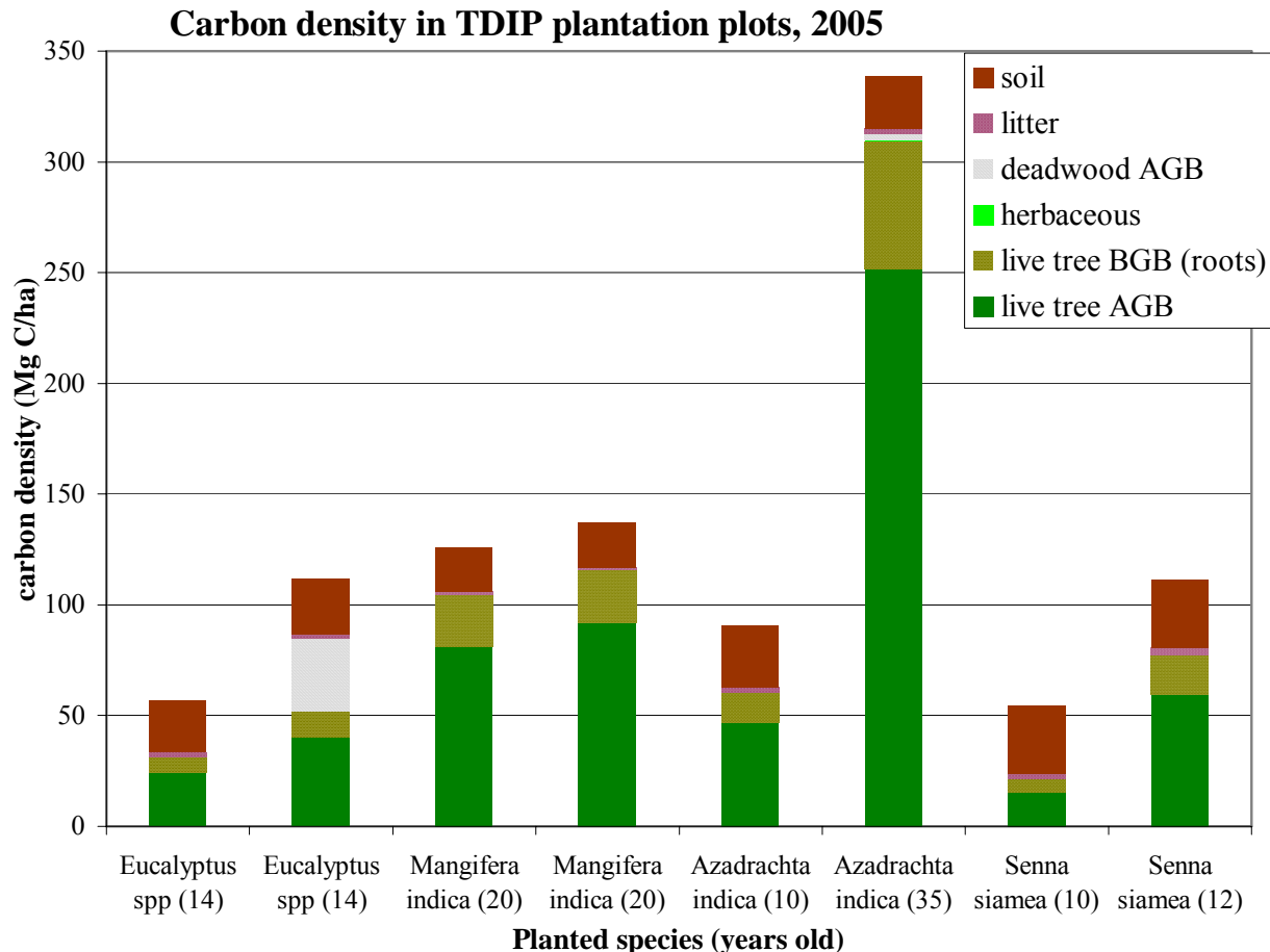
Figure 7 Carbon densities for individual sample plots in plantation areas.
