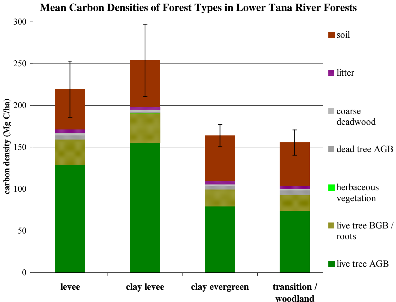
Figure 4 Carbon densities calculated as the mean density for all sample plots in a forest class. Error bars denote 95% confidence interval for the mean total carbon density (sum of all carbon pools).
