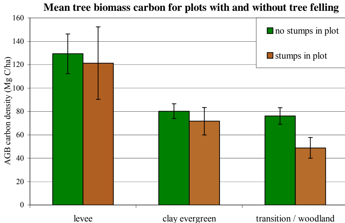
Figure 6 Carbon densities estimated from means of inventory plots in each forest type. Error bars indicate 95% confidence interval. AGB = aboveground biomass from trees
